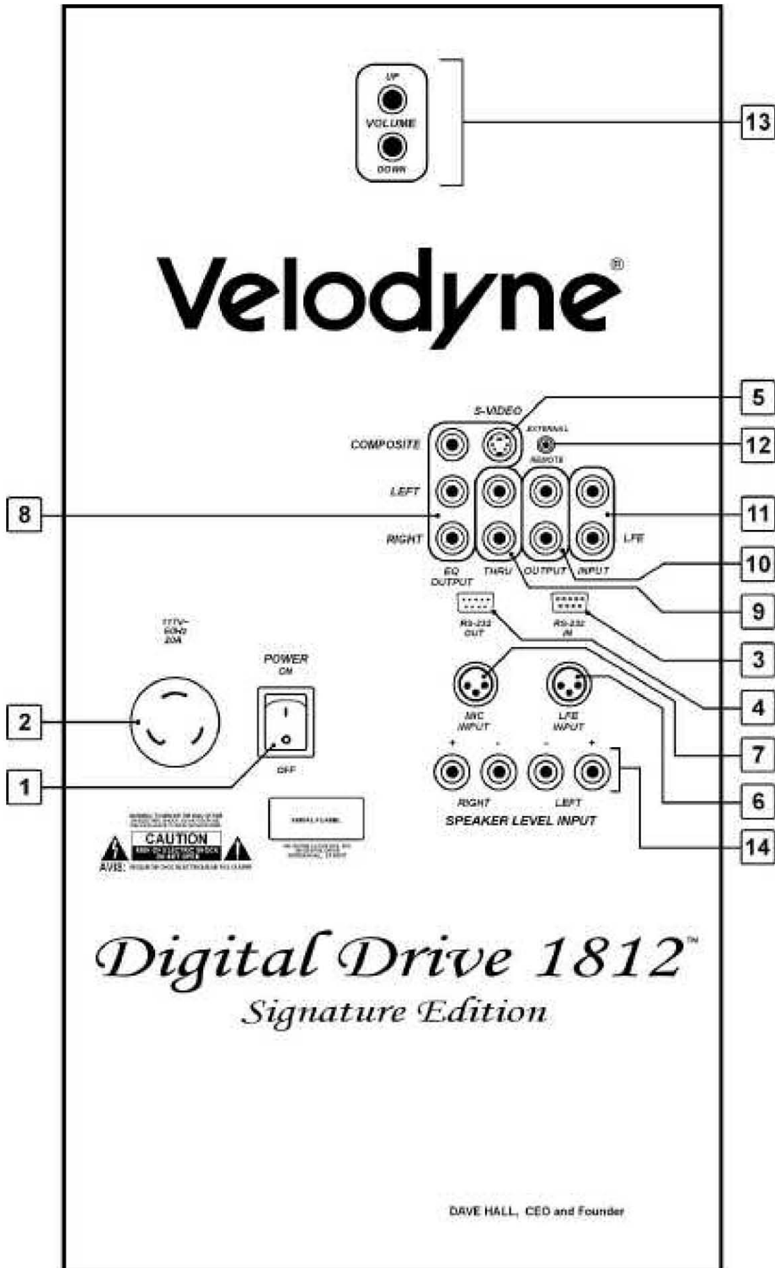
Figure 2: Digital Drive Rear Panel Connections
