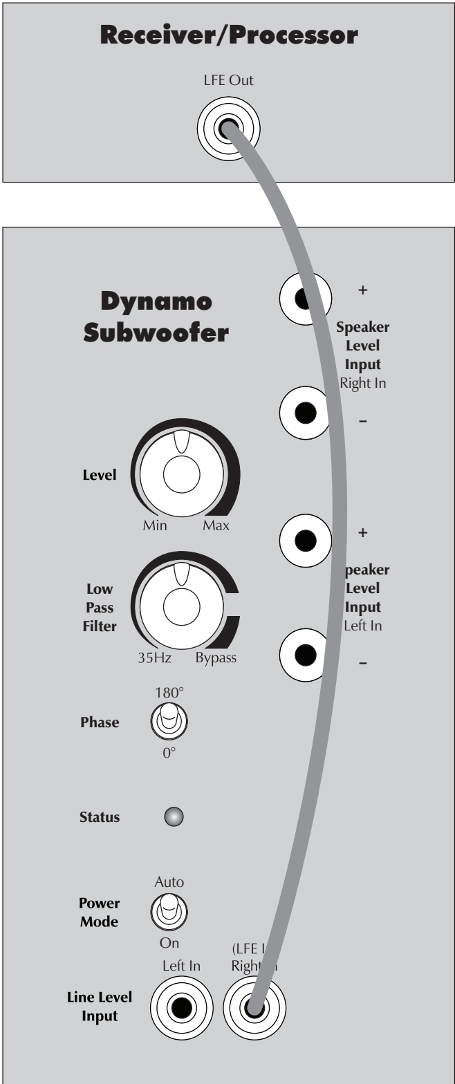
Figure 5. Signal connection for speaker level inputs.
