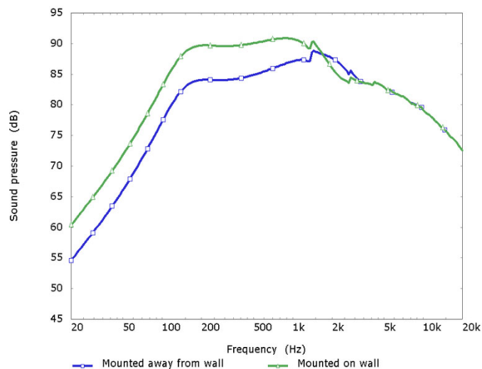
• Simulation showing the bass response boost wall effect.
