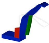
• FEA model showing the Z-Flex surround deformation as the cone moves forward.
