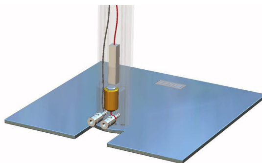
• Within the stand a small electrical circuit makes the response adjustments, terminals are located at the base for easy connection.
