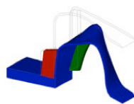
• FEA model showing the Z-Flex surround deformation as the cone moves backward.
