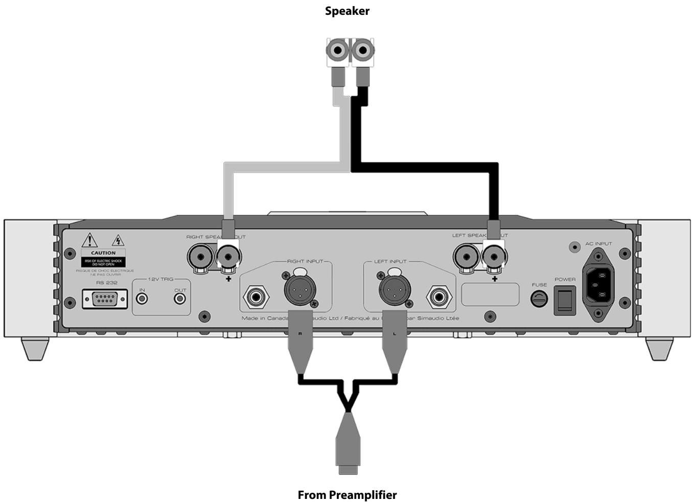
Figure 3: Bridged-Mono operation of the MOON 760A Dual-Mono Amplifier
