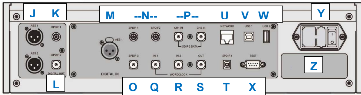
Figure 9 – Rear panel
