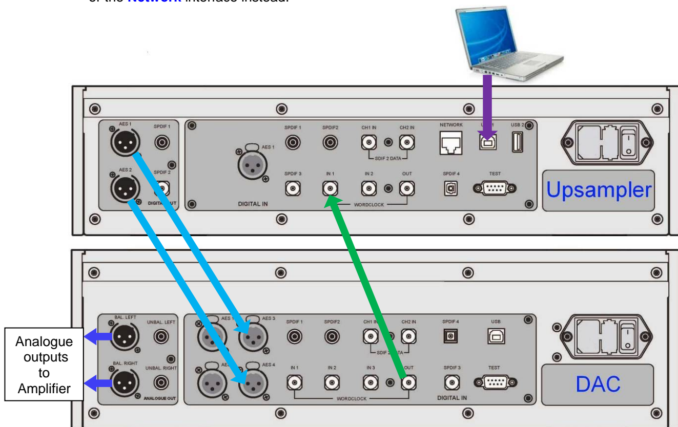
Figure 6 – Using a Vivaldi Upsampler and DAC In Universal Master Mode
