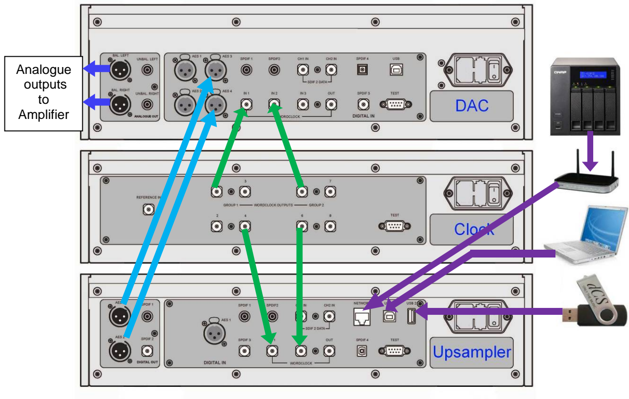
Figure 7 – Using a Vivaldi Upsampler and DAC with a Clock
