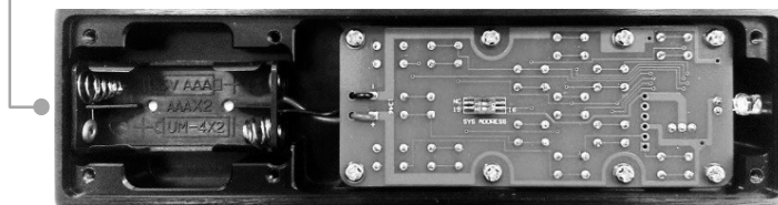
Battery compartment
